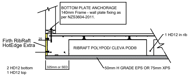
B 220mm FIRTH RIBRAFT® POLYPOD/ CLEVA POD® 140mm WALL FRAME HOTEDGE EXTRA® & UNDERSLAB INSULATION FIRTH RAFTMIX 20 OR 25MPa
