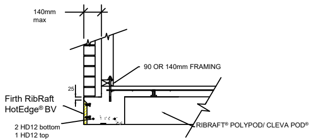
C 220mm FIRTH RIBRAFT POLYPOD/ CLEVA POD® BRICK VENEER HOTEDGE® (BV) FIRTH RAFTMIX 20 OR 25MPa
