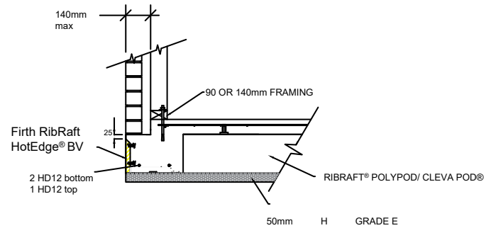
G 220mm FIRTH RIBRAFT® POLYPOD/ CLEVA POD® BRICK VENEER HOTEDGE® & UNDERSLAB INSULATION FIRTH RAFTMIX 20 OR 25MPa
