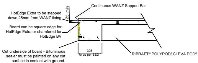
D FIRTH RIBRAFT HOTEDGE JOINERY DETAIL
